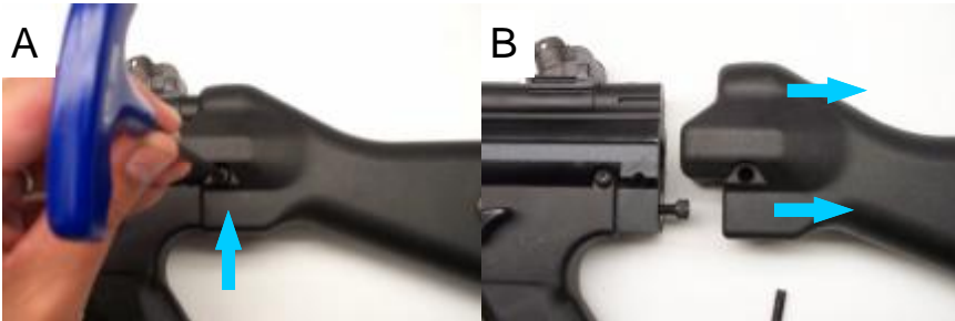
A— loosen stock retaining screw. B— Pull stock towards direction (part # 45) With a 4mm Hex tool shown.
