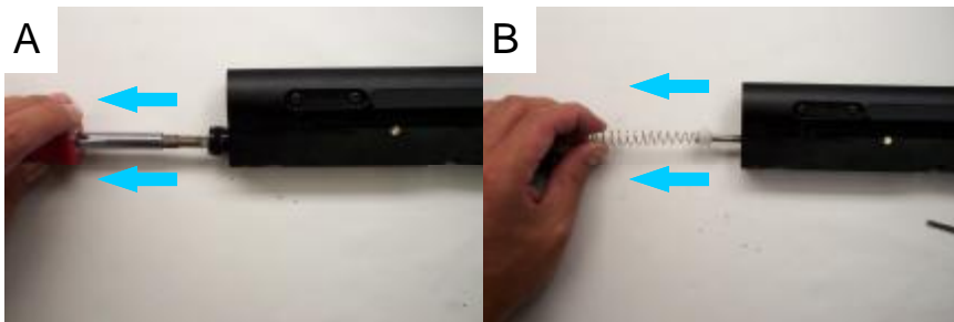
Diagram 1-7 Removing the Cup seal
