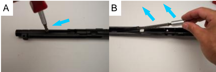
Diagram 1-11 Cocking Lever Disassembly
